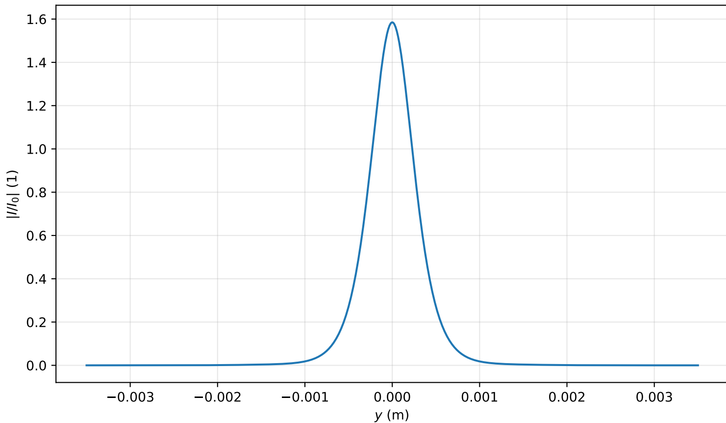
Intensity profile I(x=0, y, z=2.866)/I_0 , \text{Pin}=0.9\text{Pcr} , artificial time
